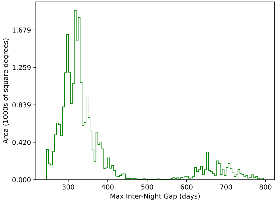
noroll_mjdp180_v3.4_10yrs All sky g band: Max Inter-Night Gap
