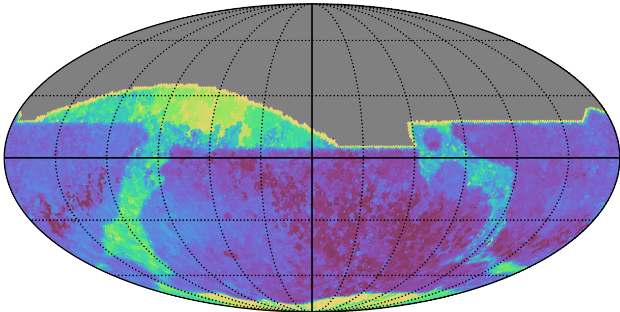
noroll_mjdp180_v3.4_10yrs All sky all bands: Max Inter-Night Gap
