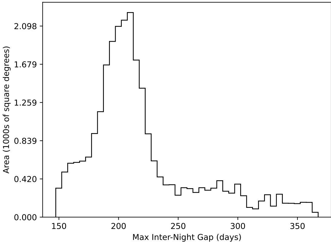
noroll_mjdp180_v3.4_10yrs All sky all bands: Max Inter-Night Gap
