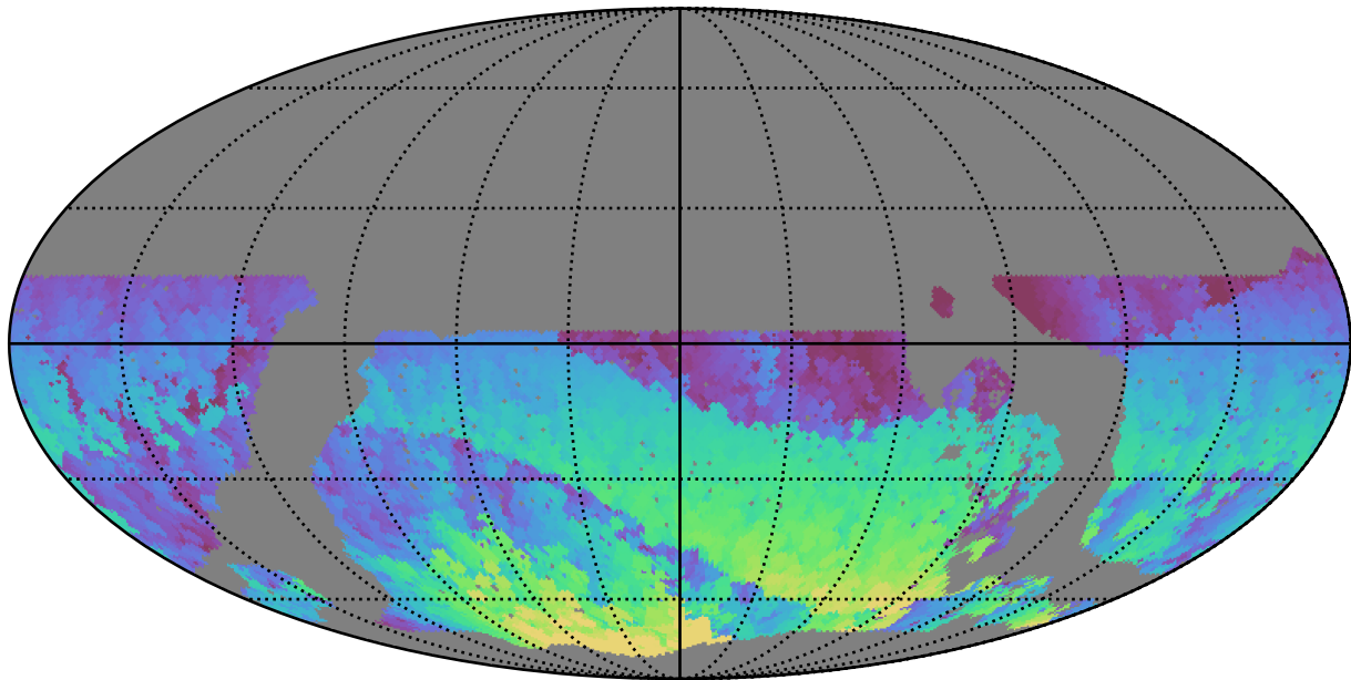
noroll_mjdp180_v3.4_10yrs WFD z band: Max HA
