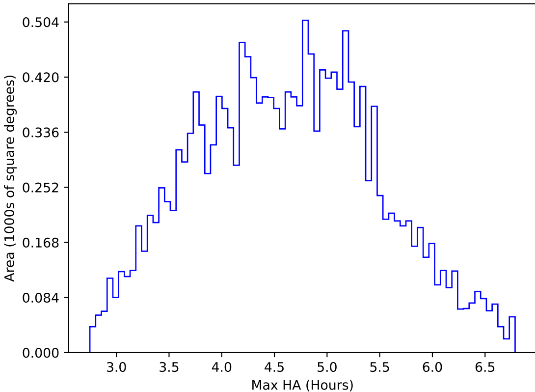
noroll_mjdp180_v3.4_10yrs WFD z band: Max HA
