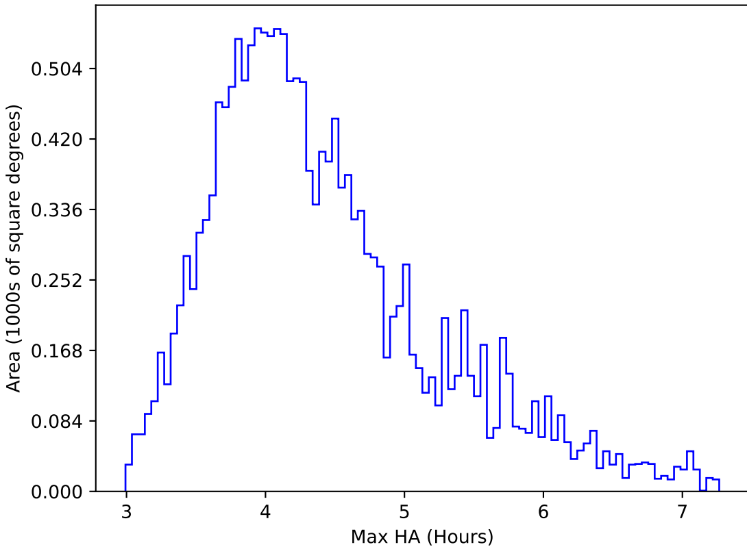
noroll_mjdp180_v3.4_10yrs WFD y band: Max HA
