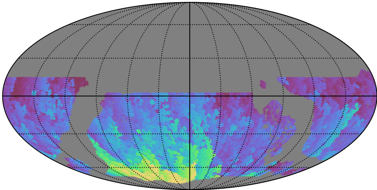
noroll_mjdp180_v3.4_10yrs WFD u band: Max HA
