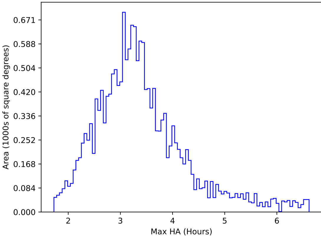
noroll_mjdp180_v3.4_10yrs WFD u band: Max HA
