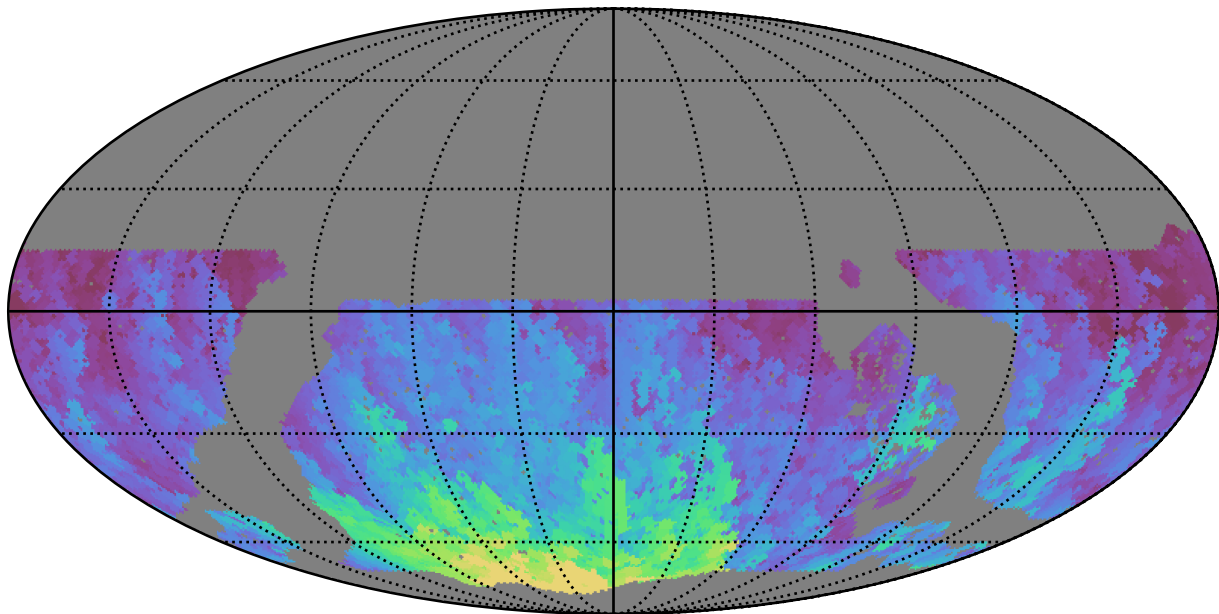
noroll_mjdp180_v3.4_10yrs WFD r band: Max HA
