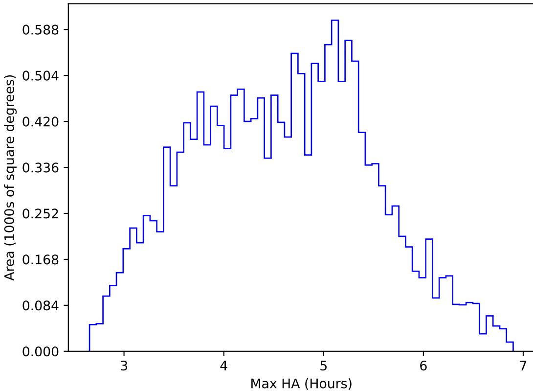
noroll_mjdp180_v3.4_10yrs WFD i band: Max HA
