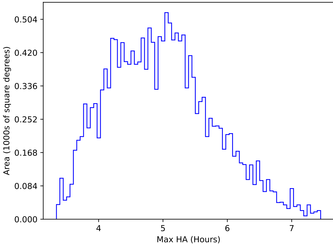
noroll_mjdp180_v3.4_10yrs WFD all bands: Max HA
