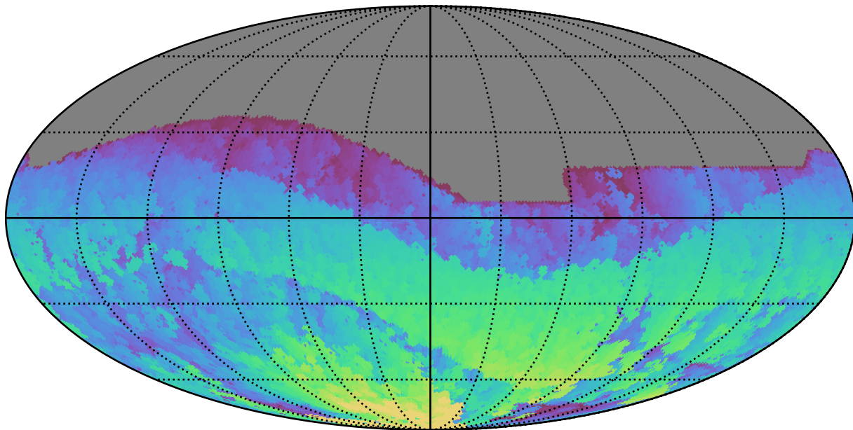
noroll_mjdp180_v3.4_10yrs All sky z band: Max HA
