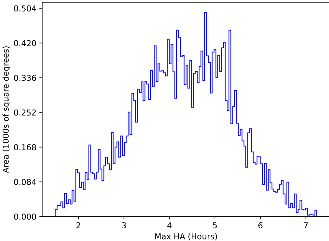
noroll_mjdp180_v3.4_10yrs All sky z band: Max HA
