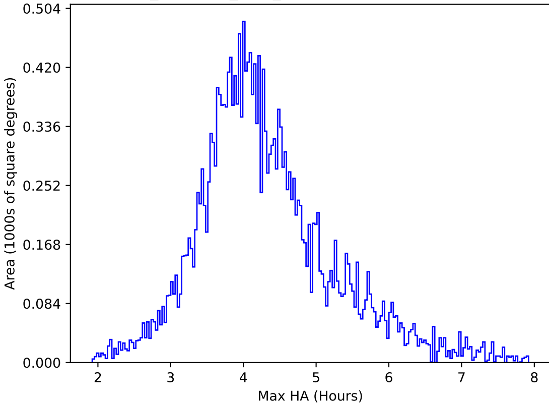
noroll_mjdp180_v3.4_10yrs All sky y band: Max HA
