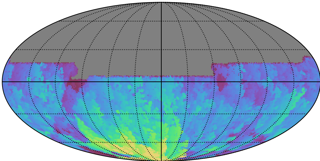
noroll_mjdp180_v3.4_10yrs All sky u band: Max HA
