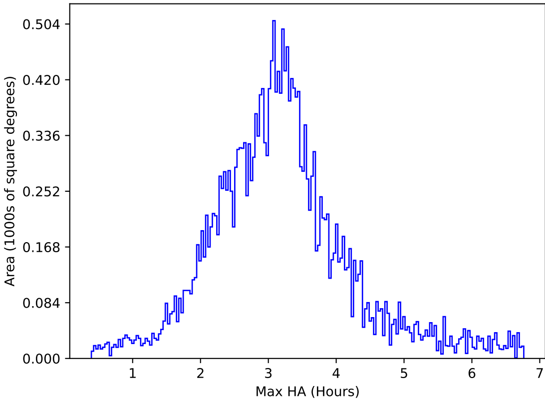
noroll_mjdp180_v3.4_10yrs All sky u band: Max HA
