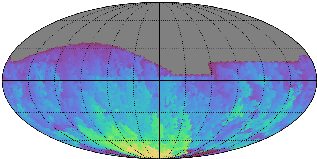
noroll_mjdp180_v3.4_10yrs All sky r band: Max HA
