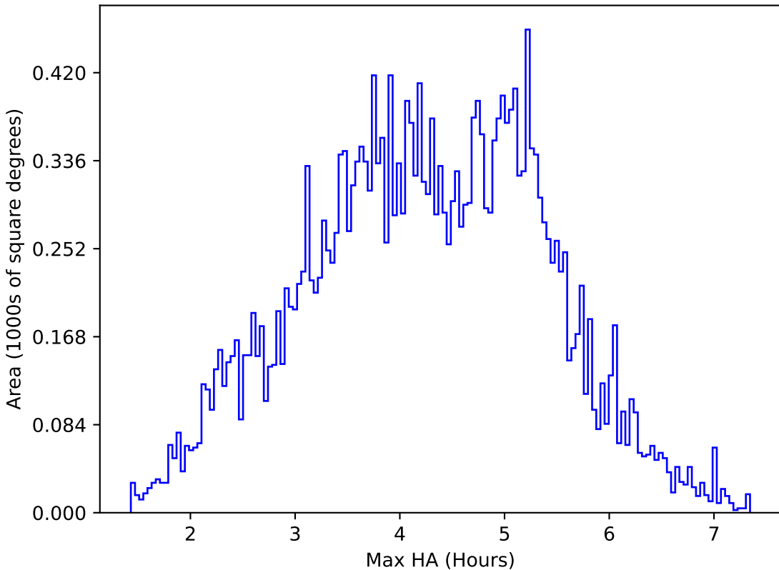
noroll_mjdp180_v3.4_10yrs All sky i band: Max HA
