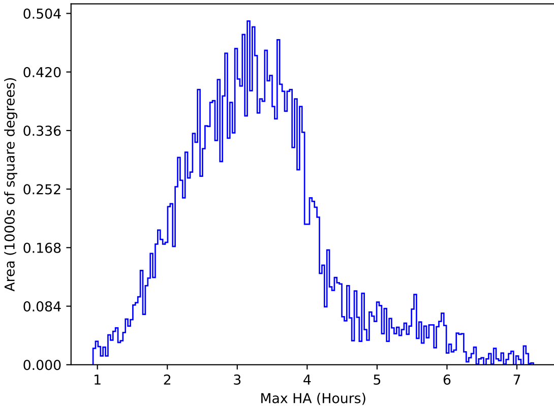
noroll_mjdp180_v3.4_10yrs All sky g band: Max HA
