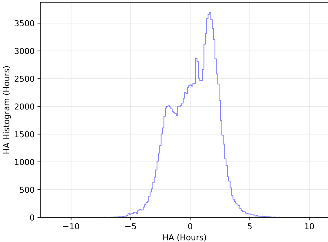
noroll_mjdp180_v3.4_10yrs WFD u band: HA Histogram
