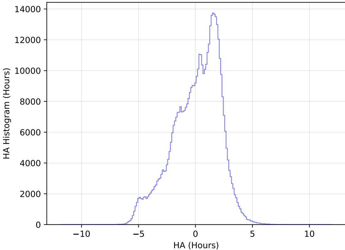
noroll_mjdp180_v3.4_10yrs WFD r band: HA Histogram
