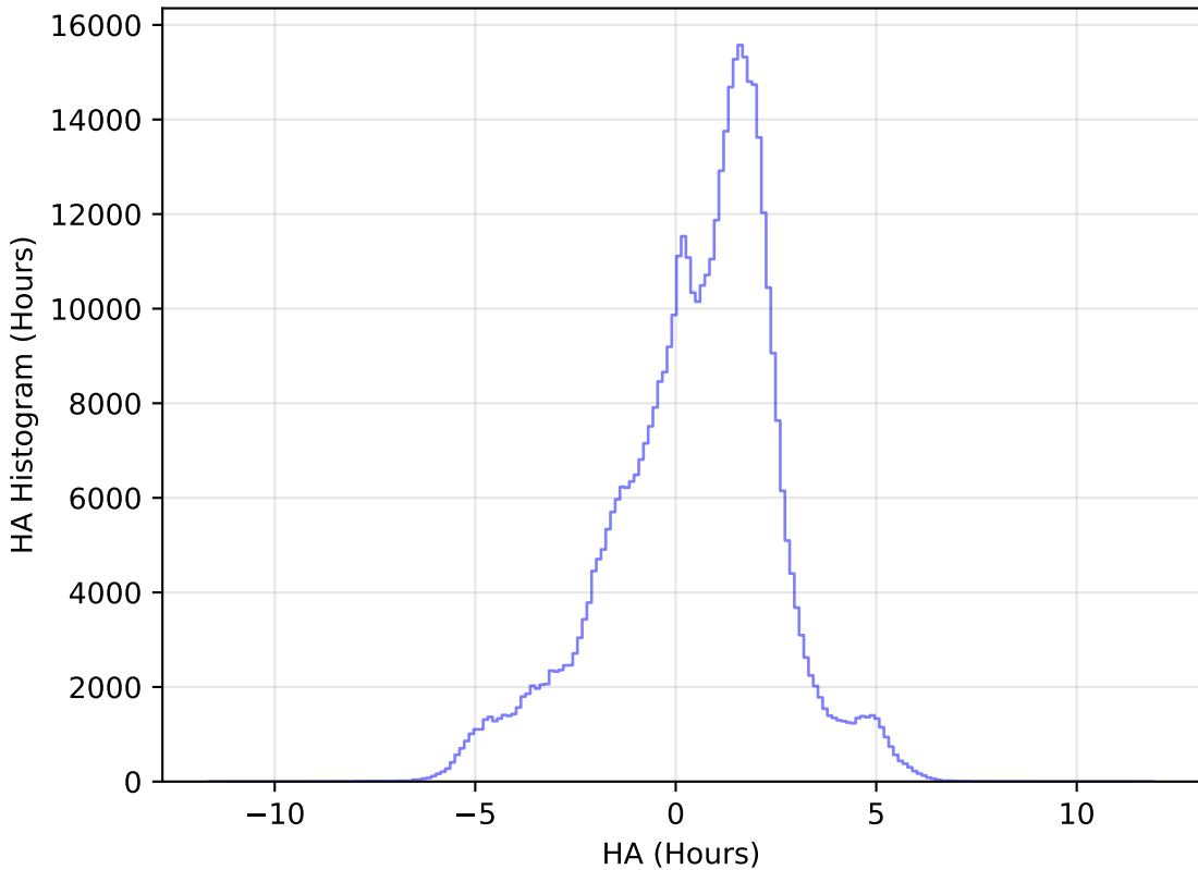
noroll_mjdp180_v3.4_10yrs WFD i band: HA Histogram
