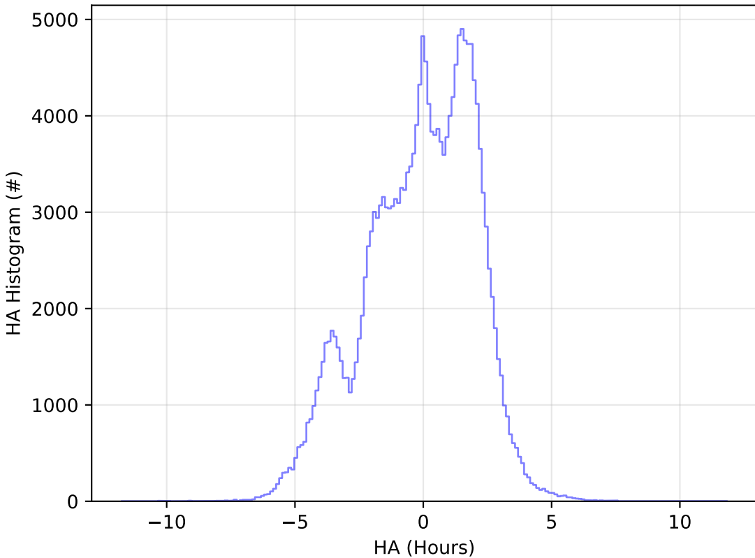
noroll_mjdp180_v3.4_10yrs WFD g band: HA Histogram
