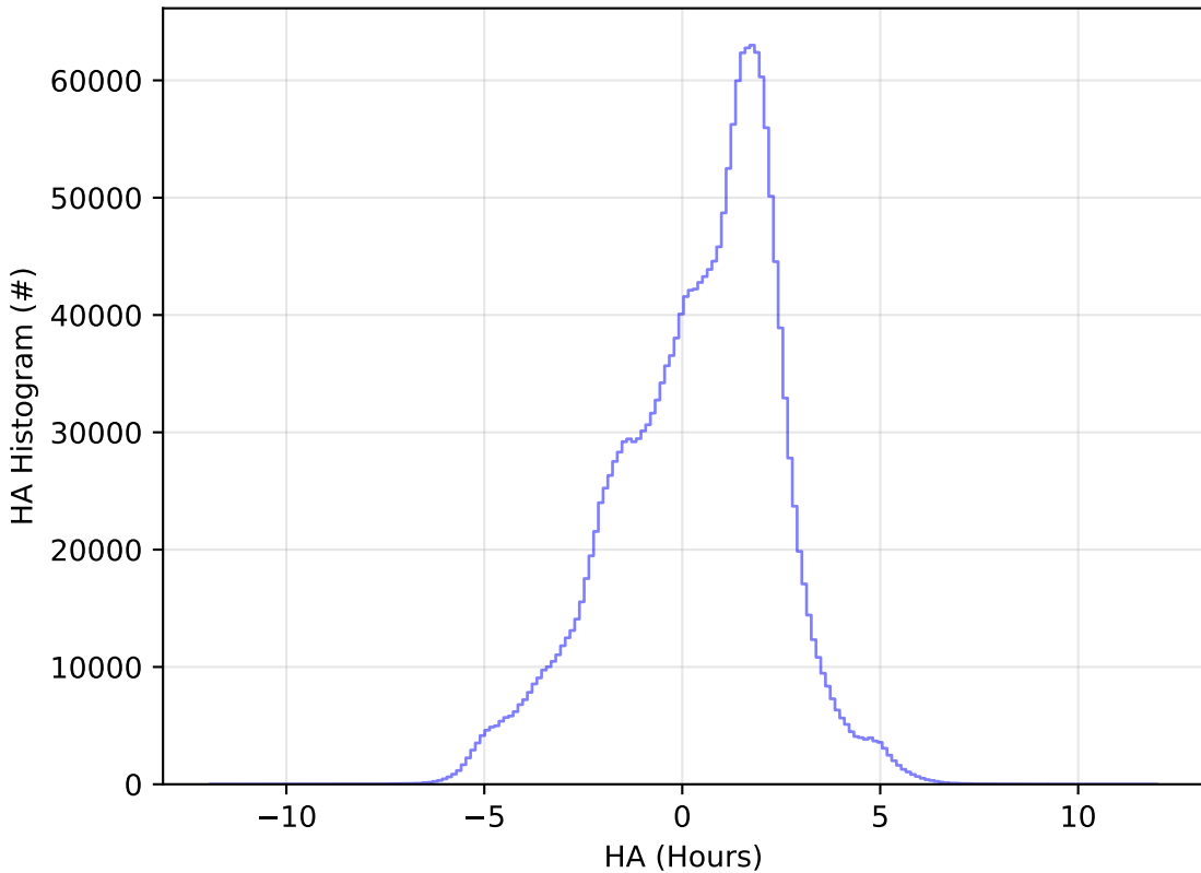
noroll_mjdp180_v3.4_10yrs WFD all bands: HA Histogram
