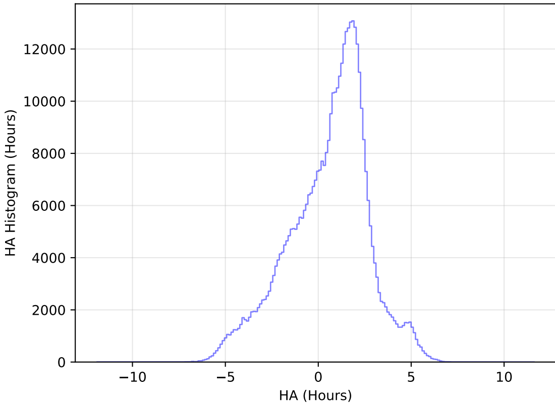
noroll_mjdp180_v3.4_10yrs All sky z band: HA Histogram
