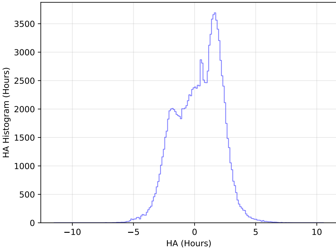
noroll_mjdp180_v3.4_10yrs All sky u band: HA Histogram
