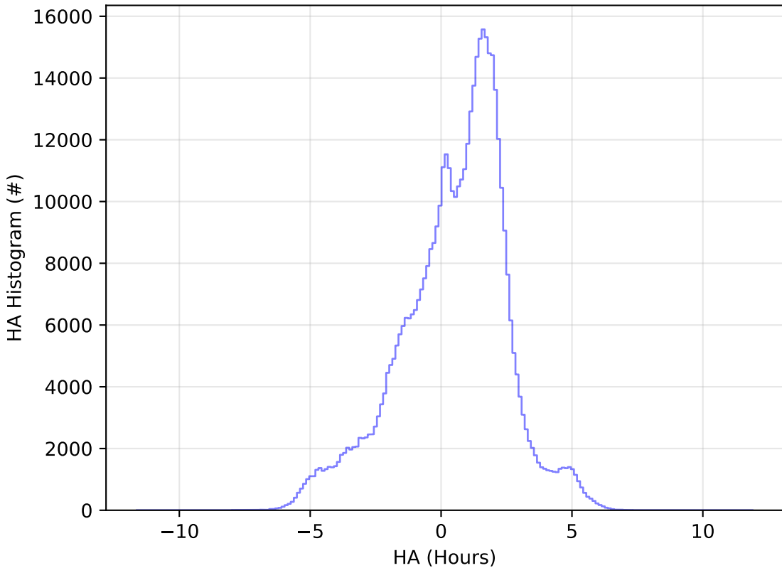
noroll_mjdp180_v3.4_10yrs All sky i band: HA Histogram
