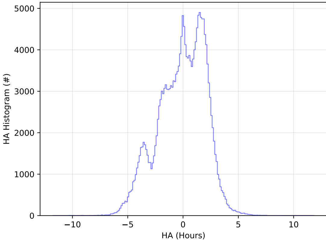
noroll_mjdp180_v3.4_10yrs All sky g band: HA Histogram
