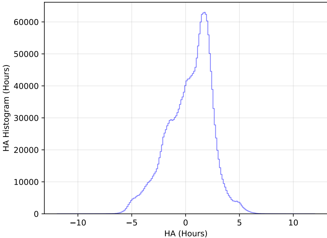
noroll_mjdp180_v3.4_10yrs All sky all bands: HA Histogram
