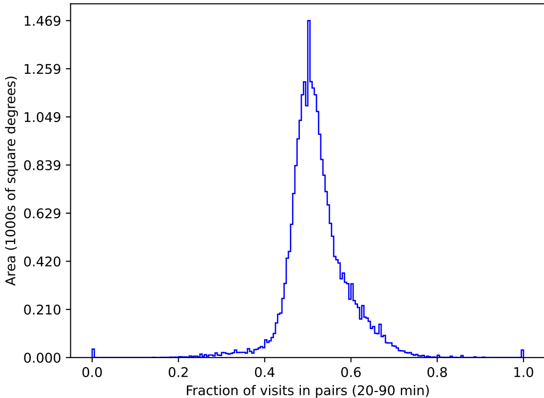
noroll_mjdp180_v3.4_10yrs gri All sky: Fraction of visits in pairs (20-90 min)
