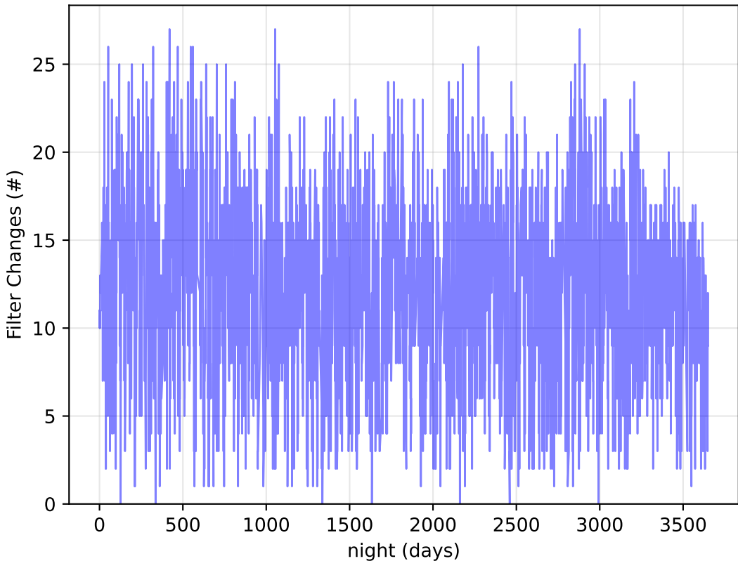
noroll_mjdp180_v3.4_10yrs Per Night: Filter Changes
