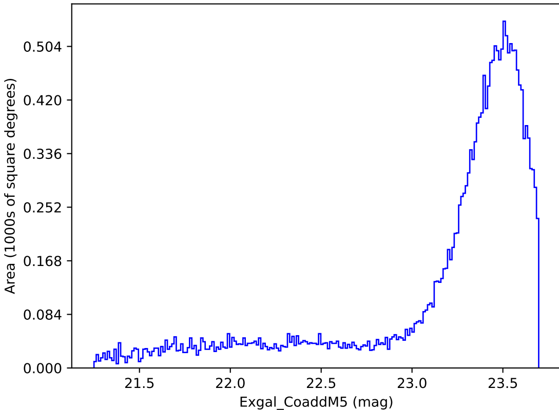
noroll_mjdp180_v3.4_10yrs Yr 3-4 y band: Exgal_CoaddM5
