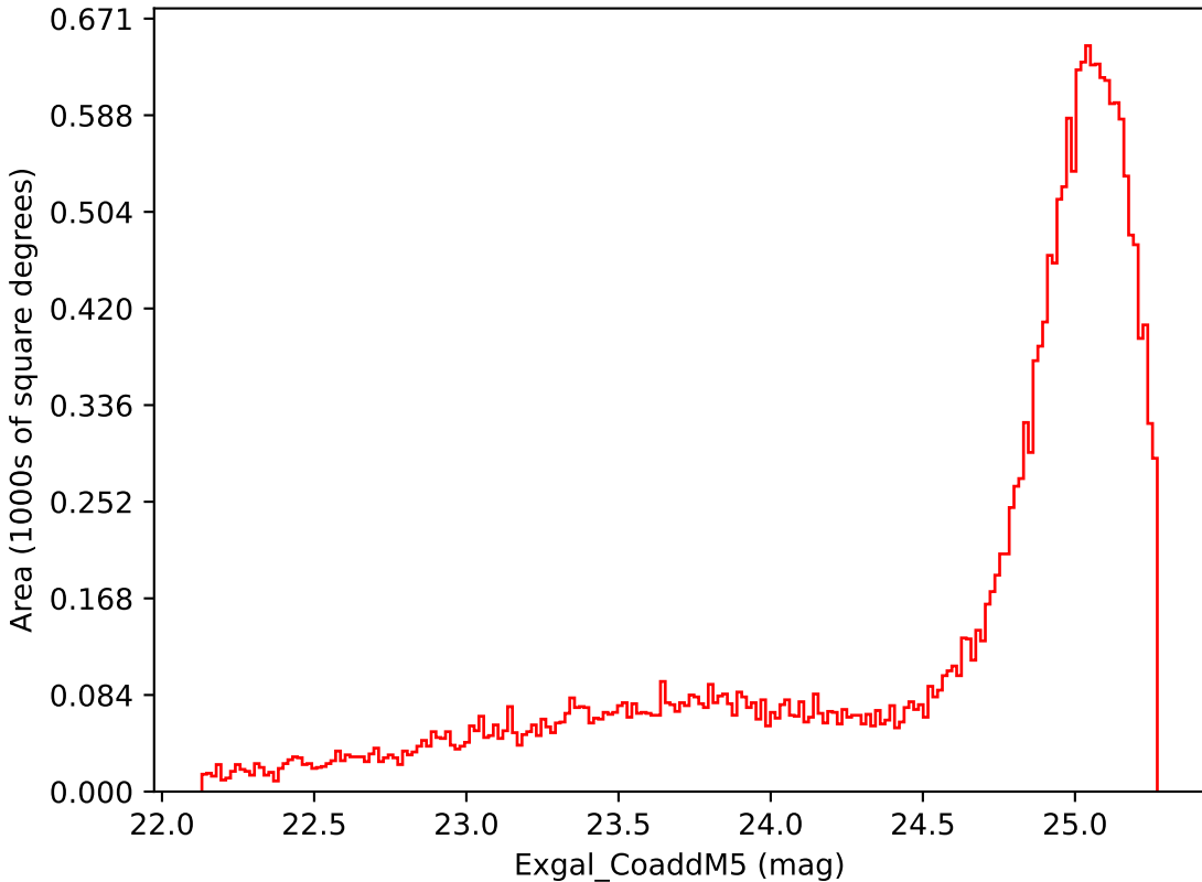
noroll_mjdp180_v3.4_10yrs Yr 3-4 i band: Exgal_CoaddM5
