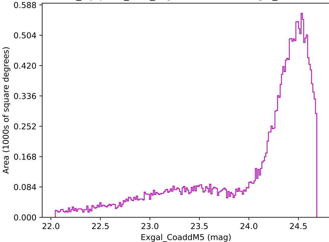
noroll_mjdp180_v3.4_10yrs Yr 1 z band: Exgal_CoaddM5
