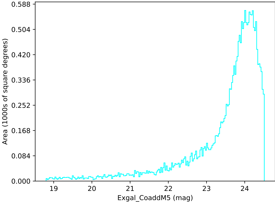
noroll_mjdp180_v3.4_10yrs Yr 1 u band: Exgal_CoaddM5
