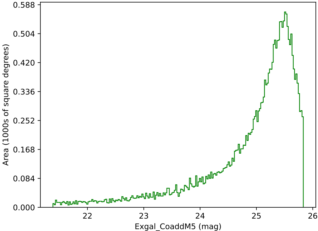
noroll_mjdp180_v3.4_10yrs Yr 1 g band: Exgal_CoaddM5
