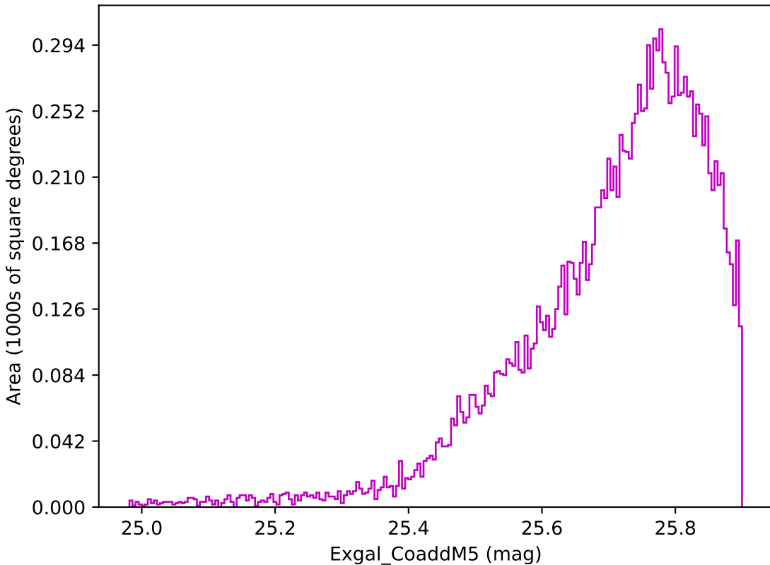
noroll_mjdp180_v3.4_10yrs WFD z band: Exgal_CoaddM5
