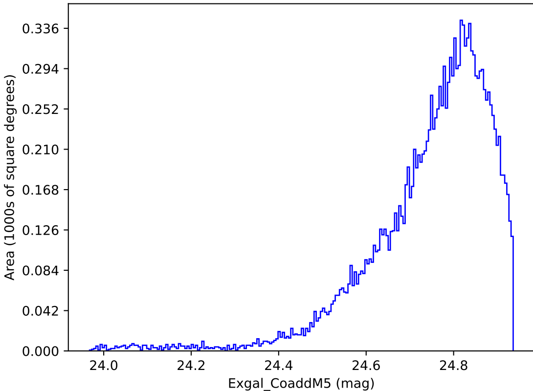
noroll_mjdp180_v3.4_10yrs WFD y band: Exgal_CoaddM5
