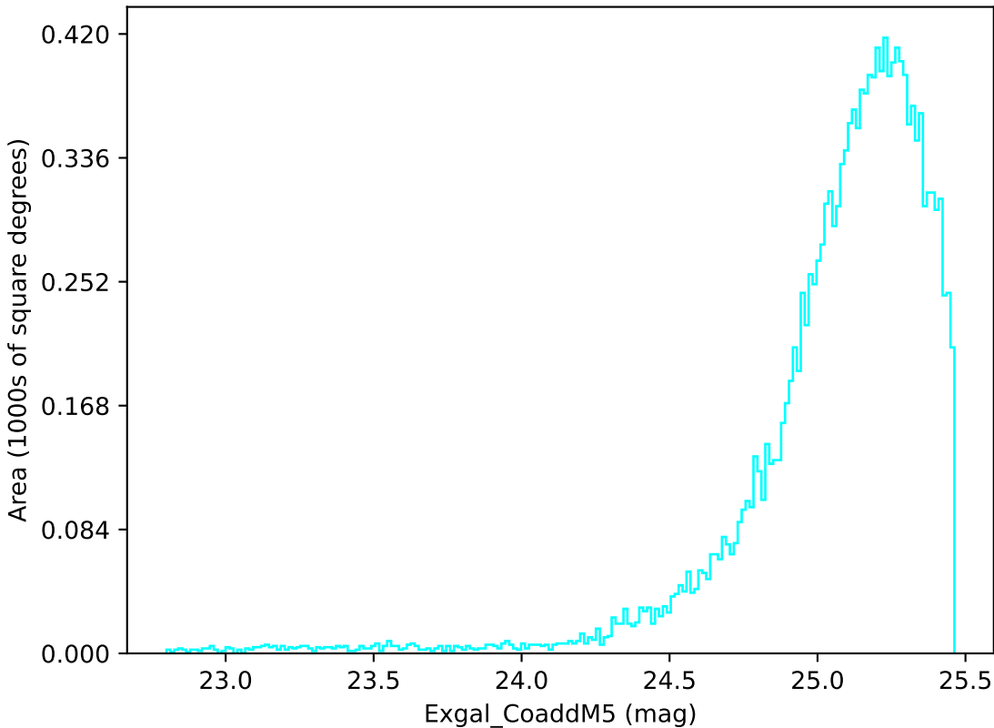
noroll_mjdp180_v3.4_10yrs WFD u band: Exgal_CoaddM5
