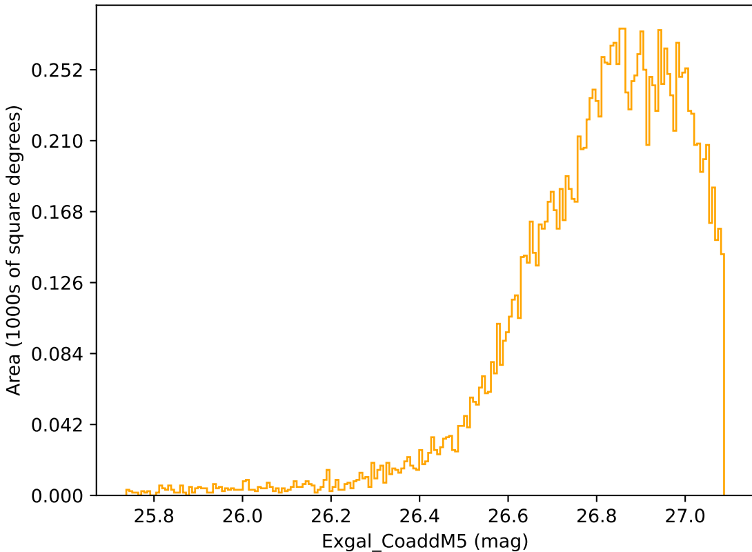
noroll_mjdp180_v3.4_10yrs WFD r band: Exgal_CoaddM5
