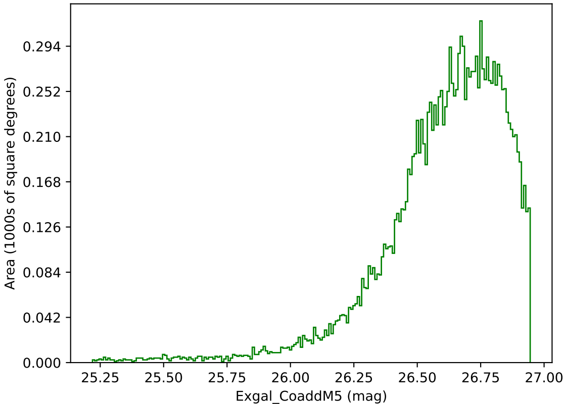
noroll_mjdp180_v3.4_10yrs WFD g band: Exgal_CoaddM5
