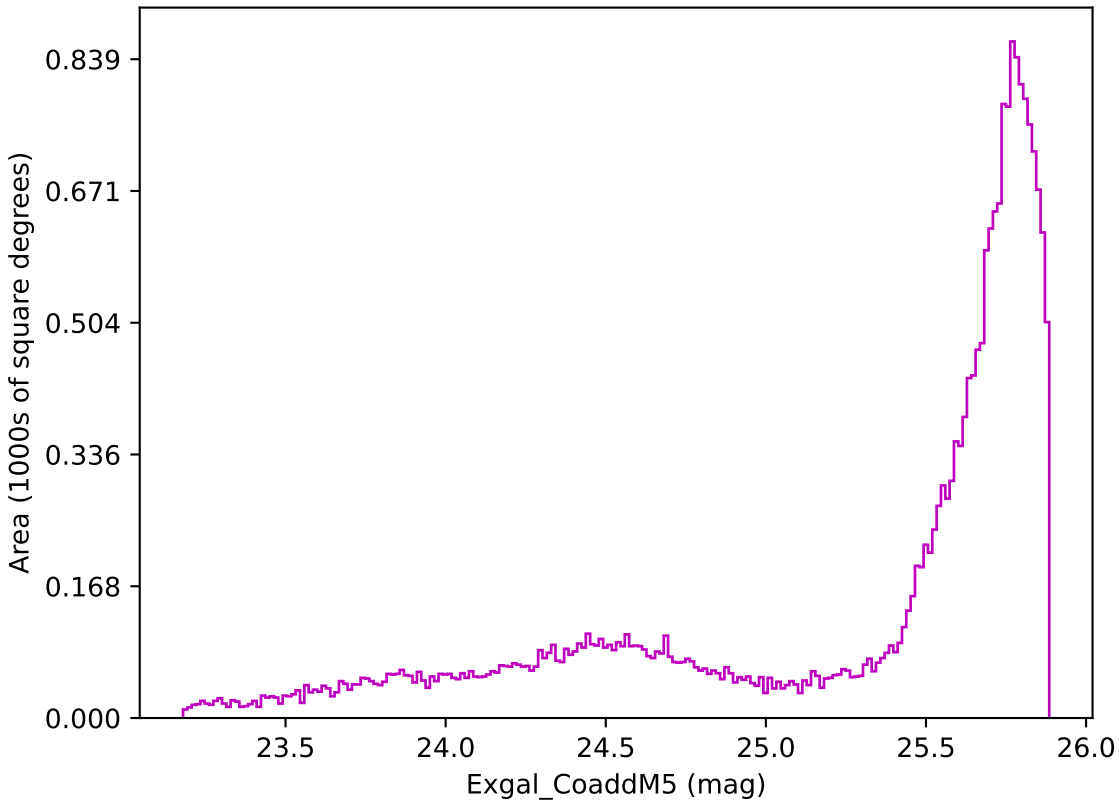
noroll_mjdp180_v3.4_10yrs All sky z band: Exgal_CoaddM5
