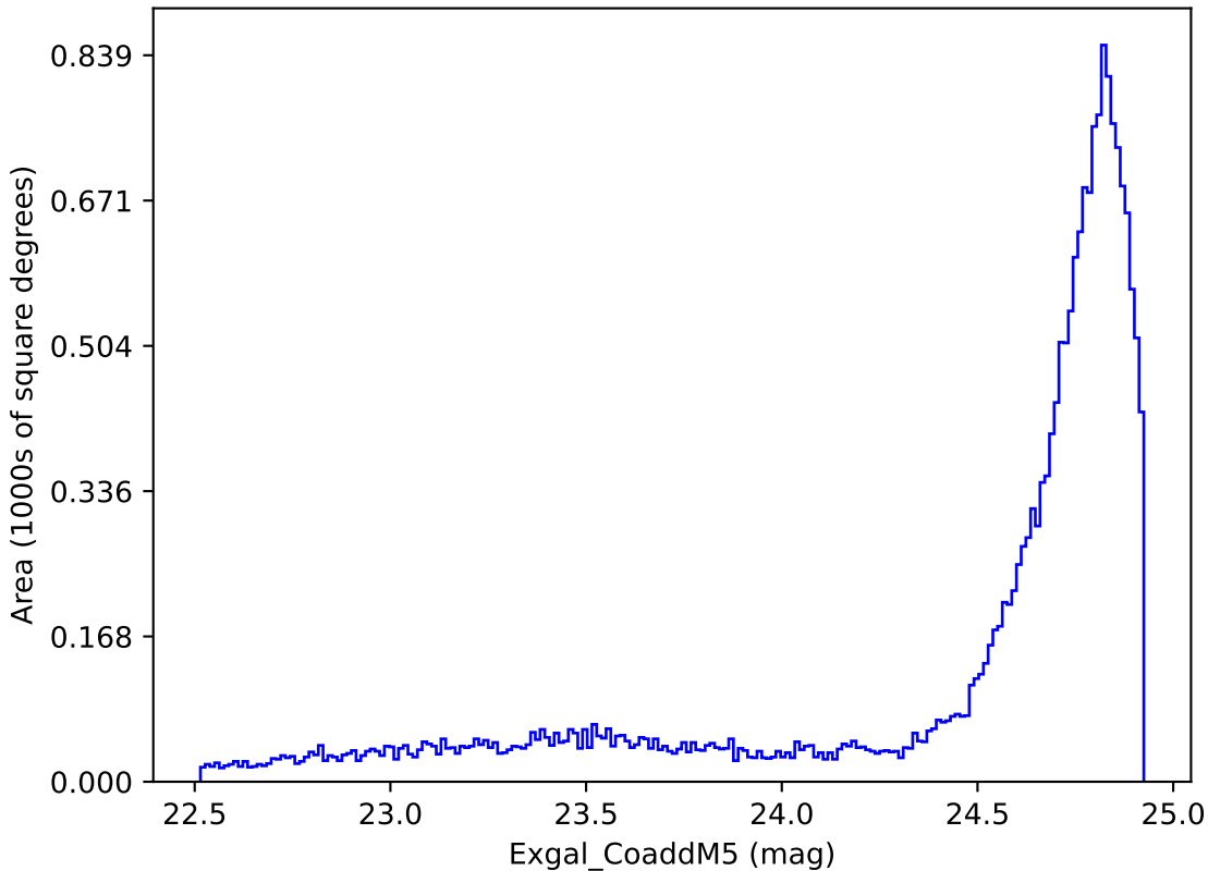
noroll_mjdp180_v3.4_10yrs All sky y band: Exgal_CoaddM5
