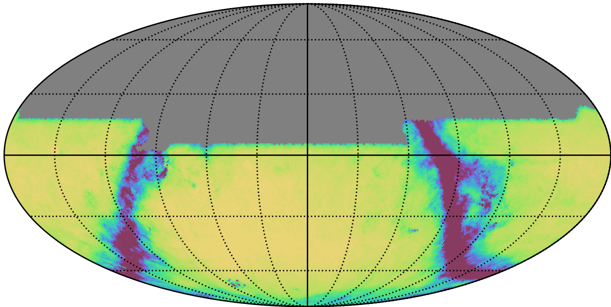
noroll_mjdp180_v3.4_10yrs All sky u band: Exgal_CoaddM5
