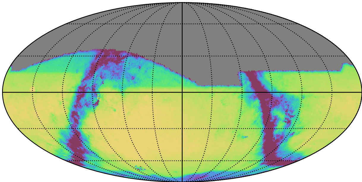
noroll_mjdp180_v3.4_10yrs All sky r band: Exgal_CoaddM5
