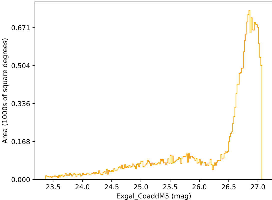
noroll_mjdp180_v3.4_10yrs All sky r band: Exgal_CoaddM5
