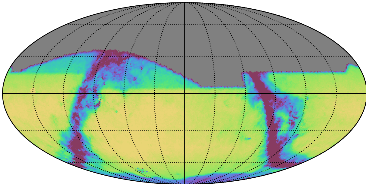
noroll_mjdp180_v3.4_10yrs All sky i band: Exgal_CoaddM5
