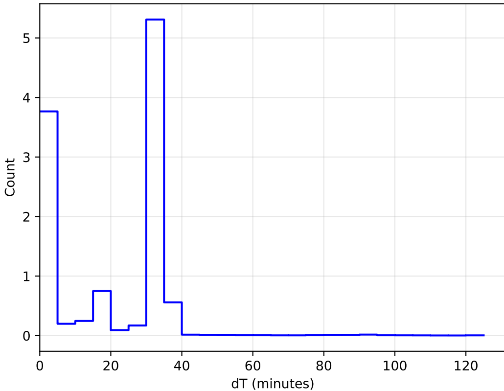
1e6 noroll_mjdp180_v3.4_10yrs WFD: DeltaT Histogram
