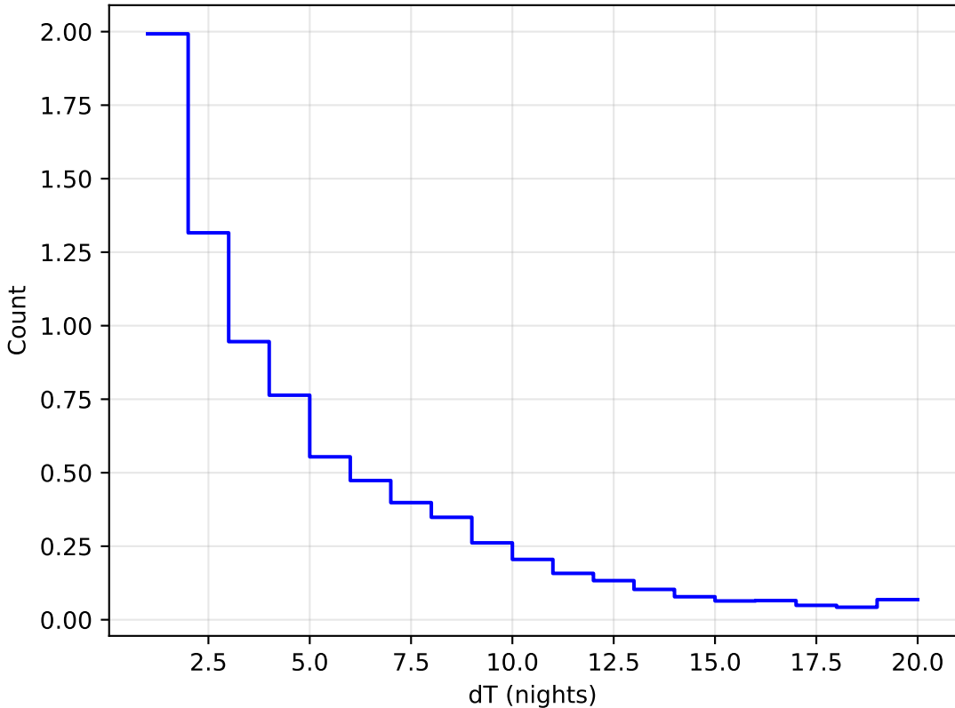
noroll_mjdp180_v3.4_10yrs WFD all bands: DeltaNight Histogram
