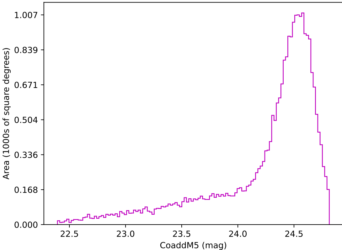
noroll_mjdp180_v3.4_10yrs Yr 3-4 z band: CoaddM5
